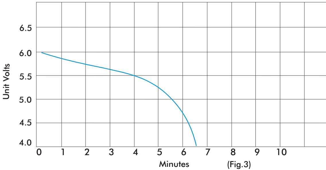
Typical Voltage Curve on Sustained Cranking at 27°C, 1.250(27°C) and 4HMFG 31KP at a Current of 1400A
