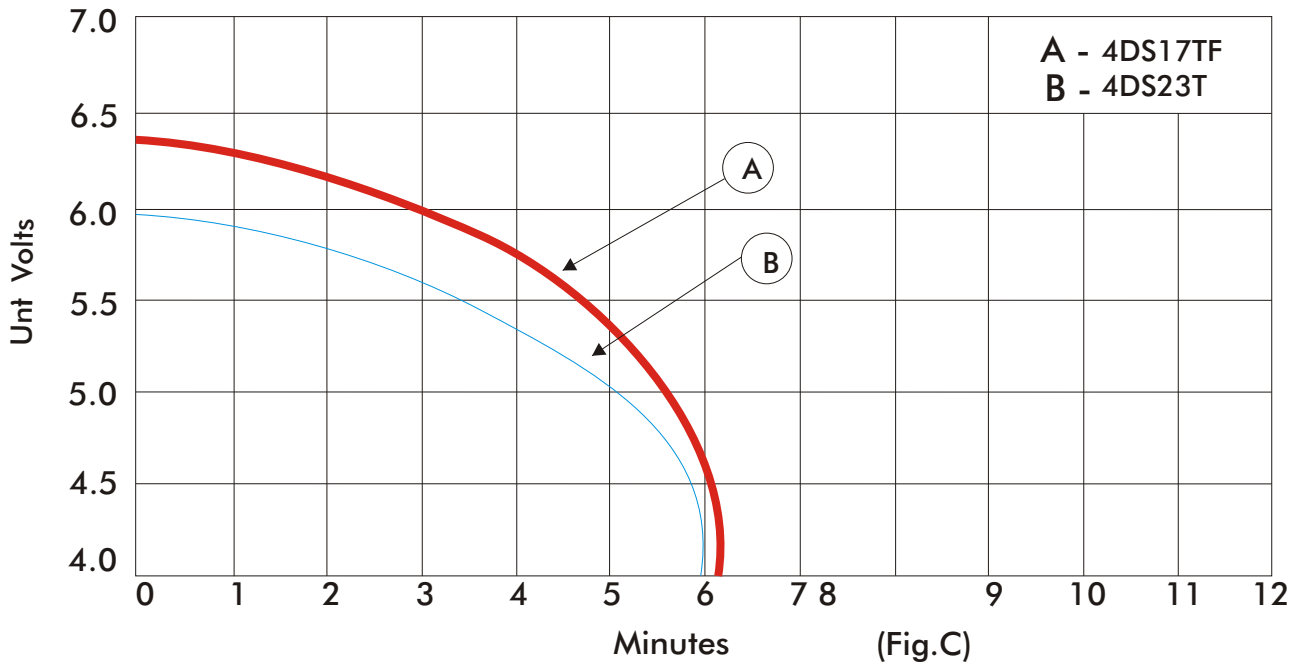
Typical Voltage Curves on Sustained Cranking at 27°C, 1.250(27°C) 4DS17TF at a current of 940A & 4DS23T at a Current of 1400A
