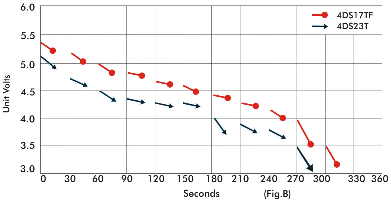
Typical Voltage Curves on Initial Cranking at 27°C, 1.250(27°C) 4DS17TF at a current of 1500A & 4DS23T at a Current of 2300A
